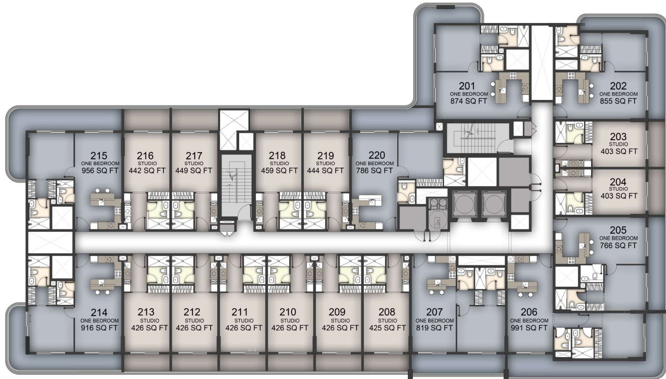
2ND FLOOR PLAN
