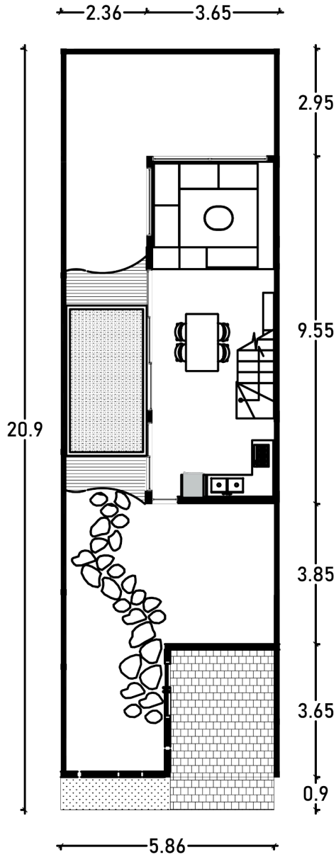
Ground Floor
