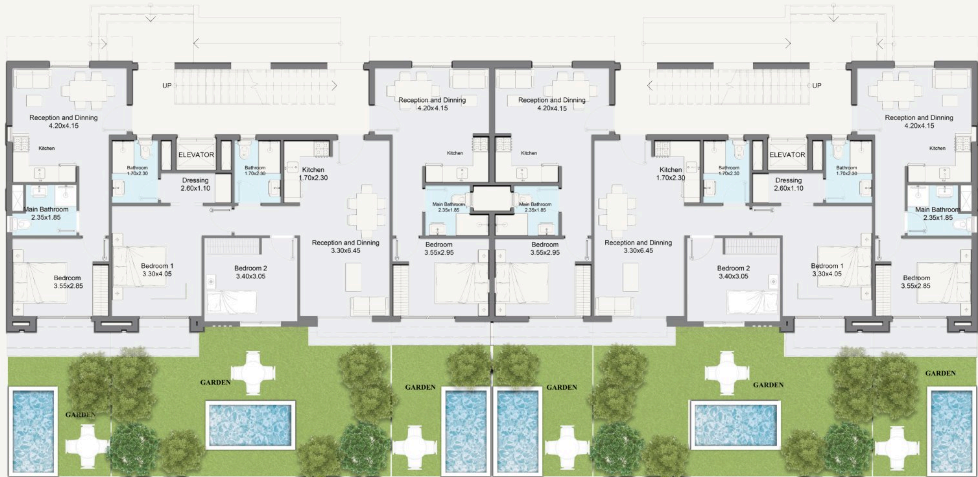
Ground Floor
