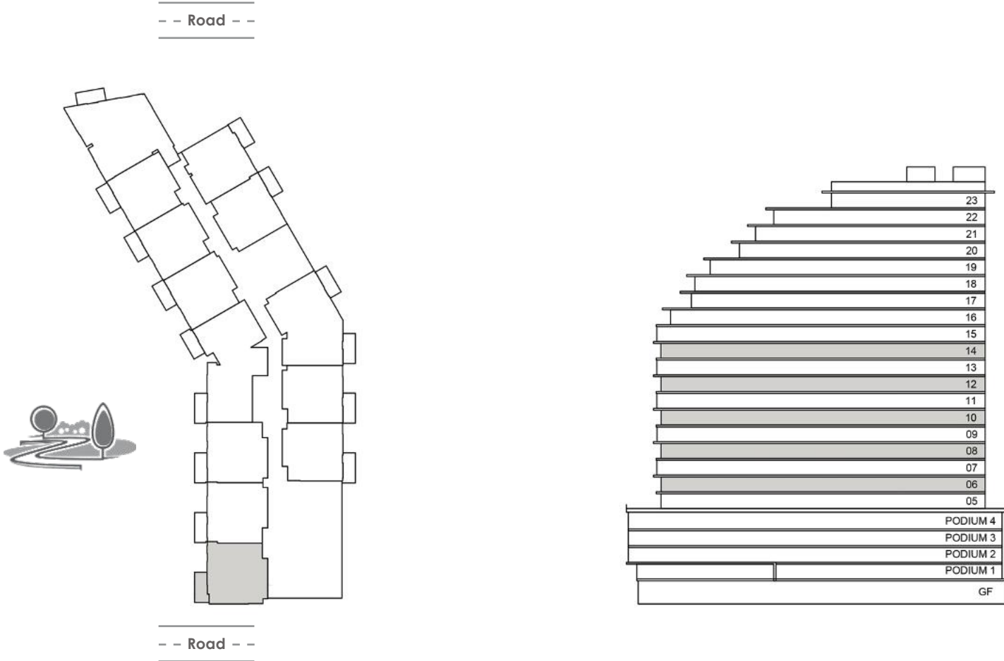
KEY SECTION
