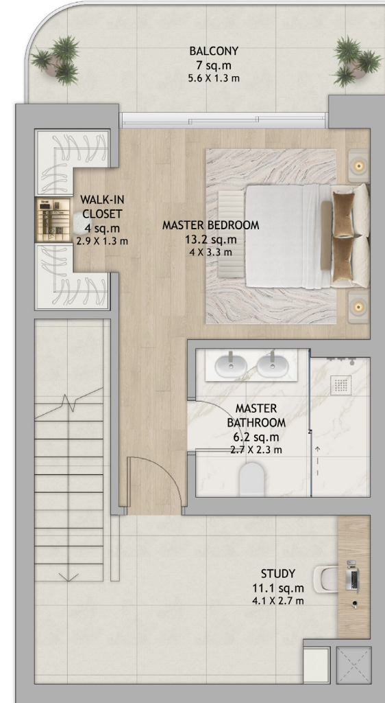
Upper Floor
