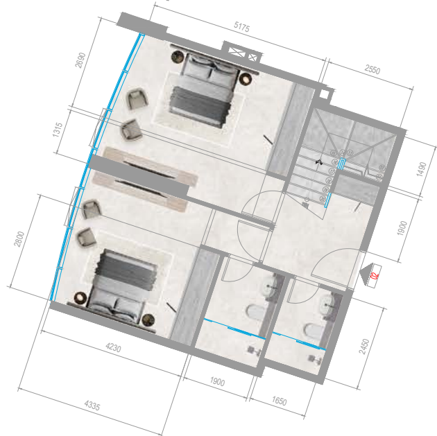
FIRST FLOOR LEVEL
