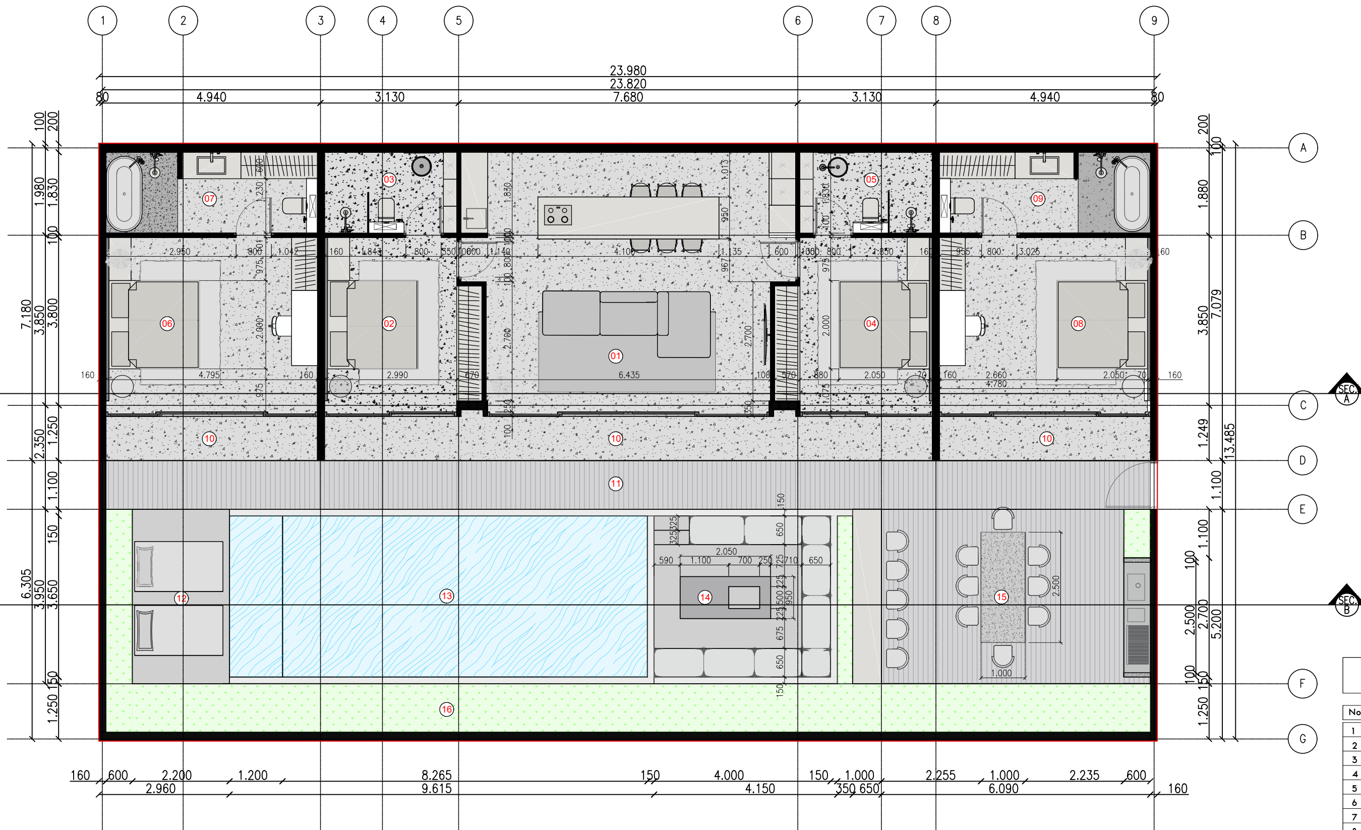
KABAKABA CASCADE. VILLA 4BR PLAN 1:100
