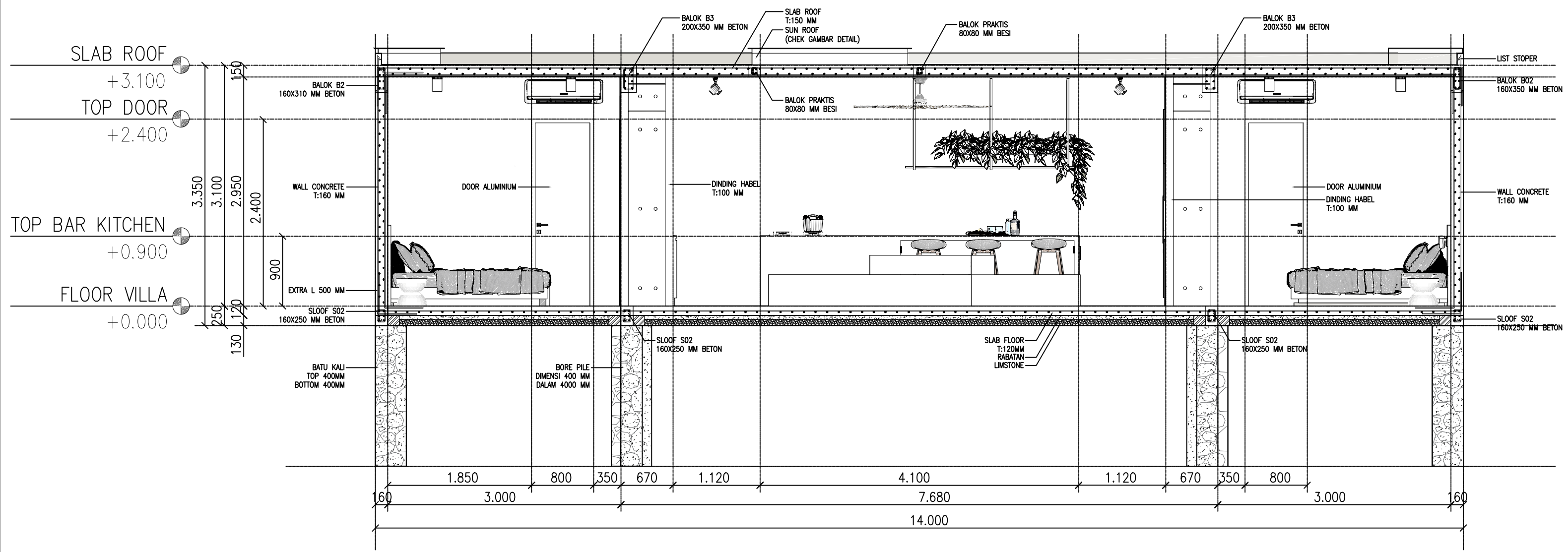
KABAKABA CASCADE. SECTION A 1:100
