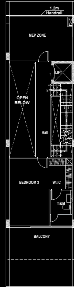
Second Floor
