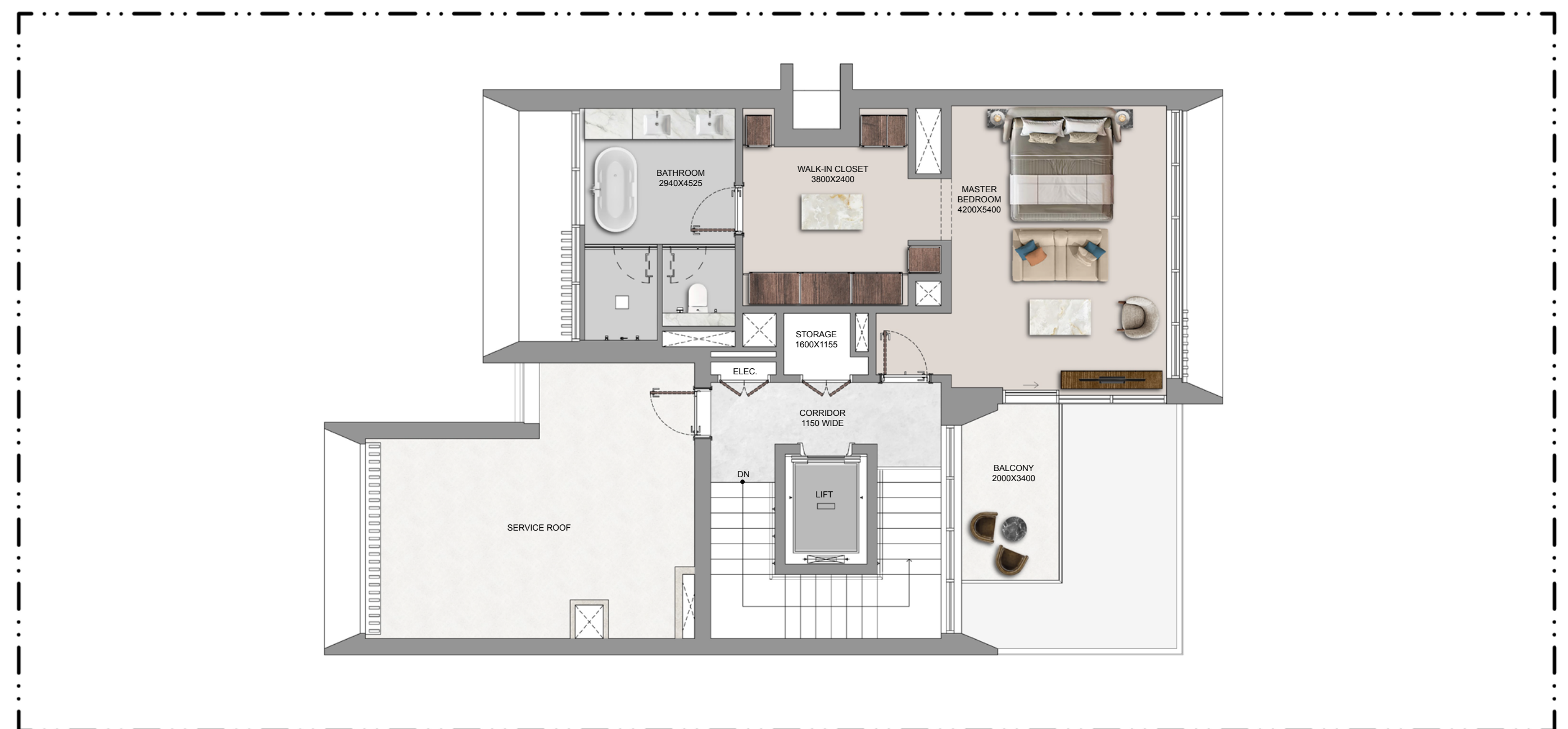
SECOND FLOOR
