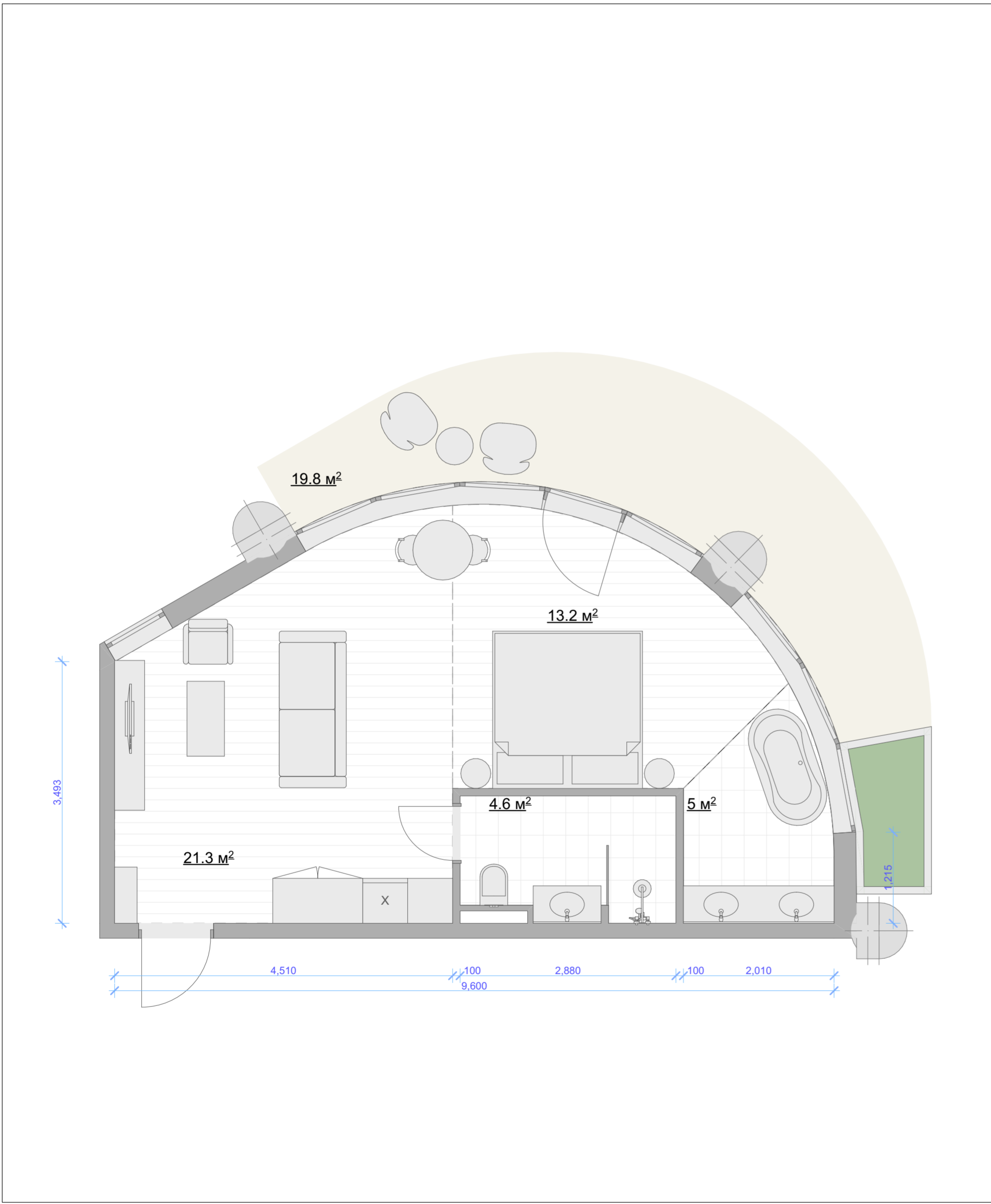
Luxe room. Type 4 x2 44,1m2 88,2m2
