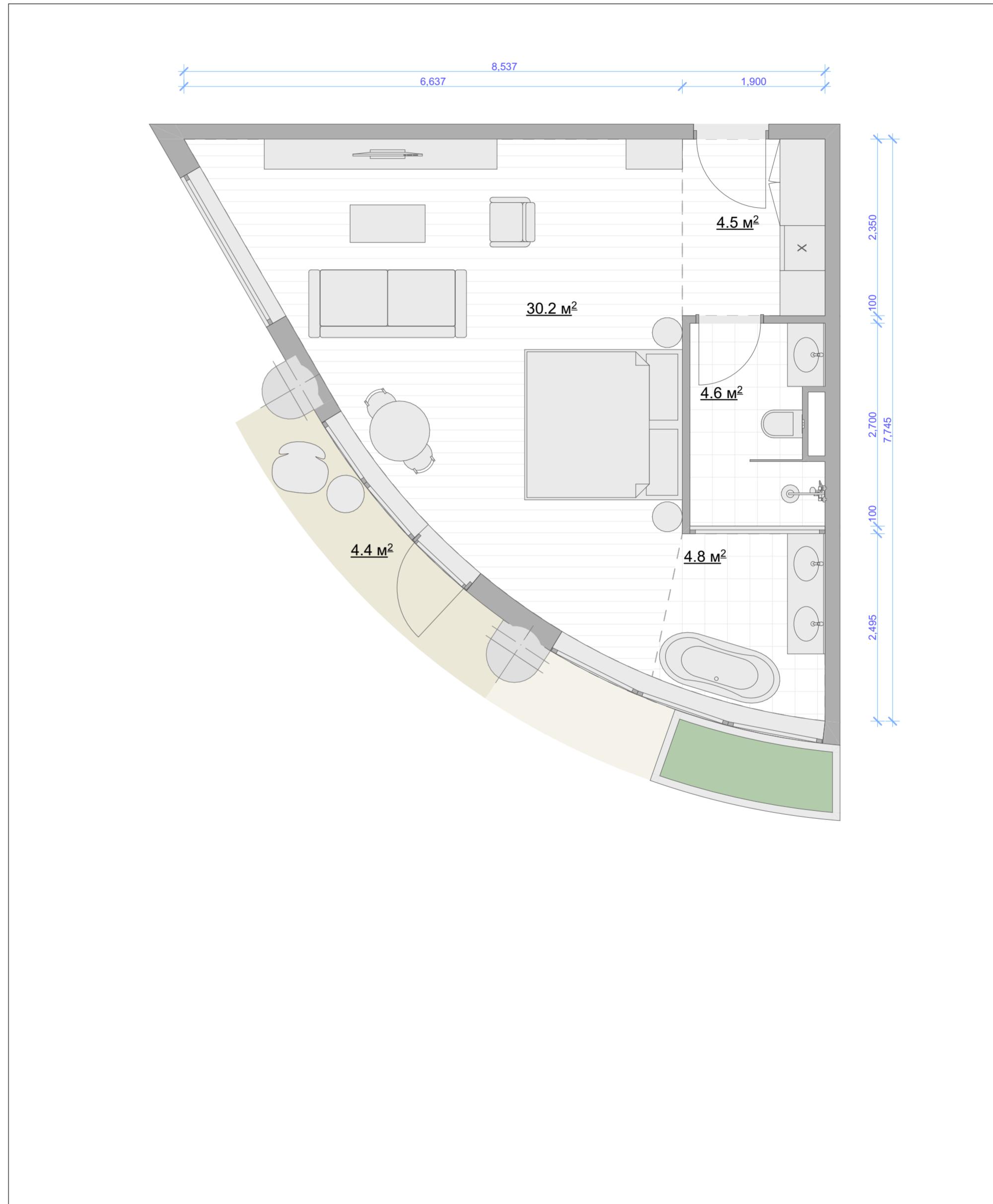
Luxe room. Type 2 x3 44,1m 2 132,3m 2
