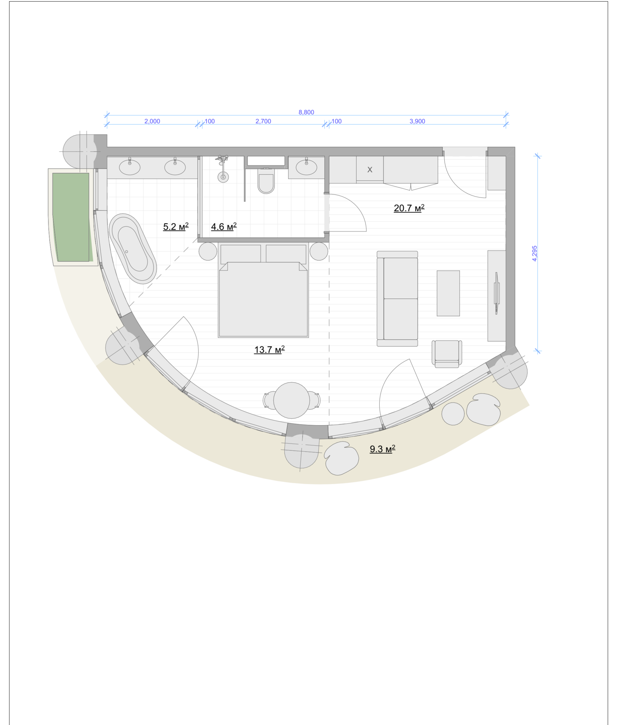
Luxe room. Type 1 44,2m 2
