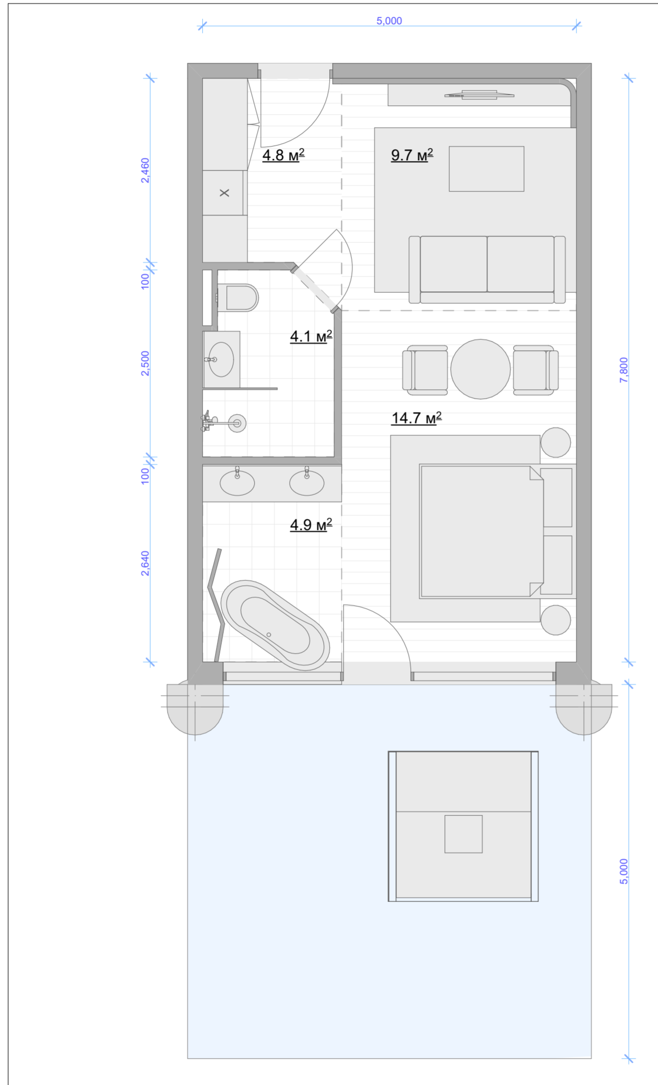
Deluxe room. Type 1 x3 38,2m 2 114,6m 2
