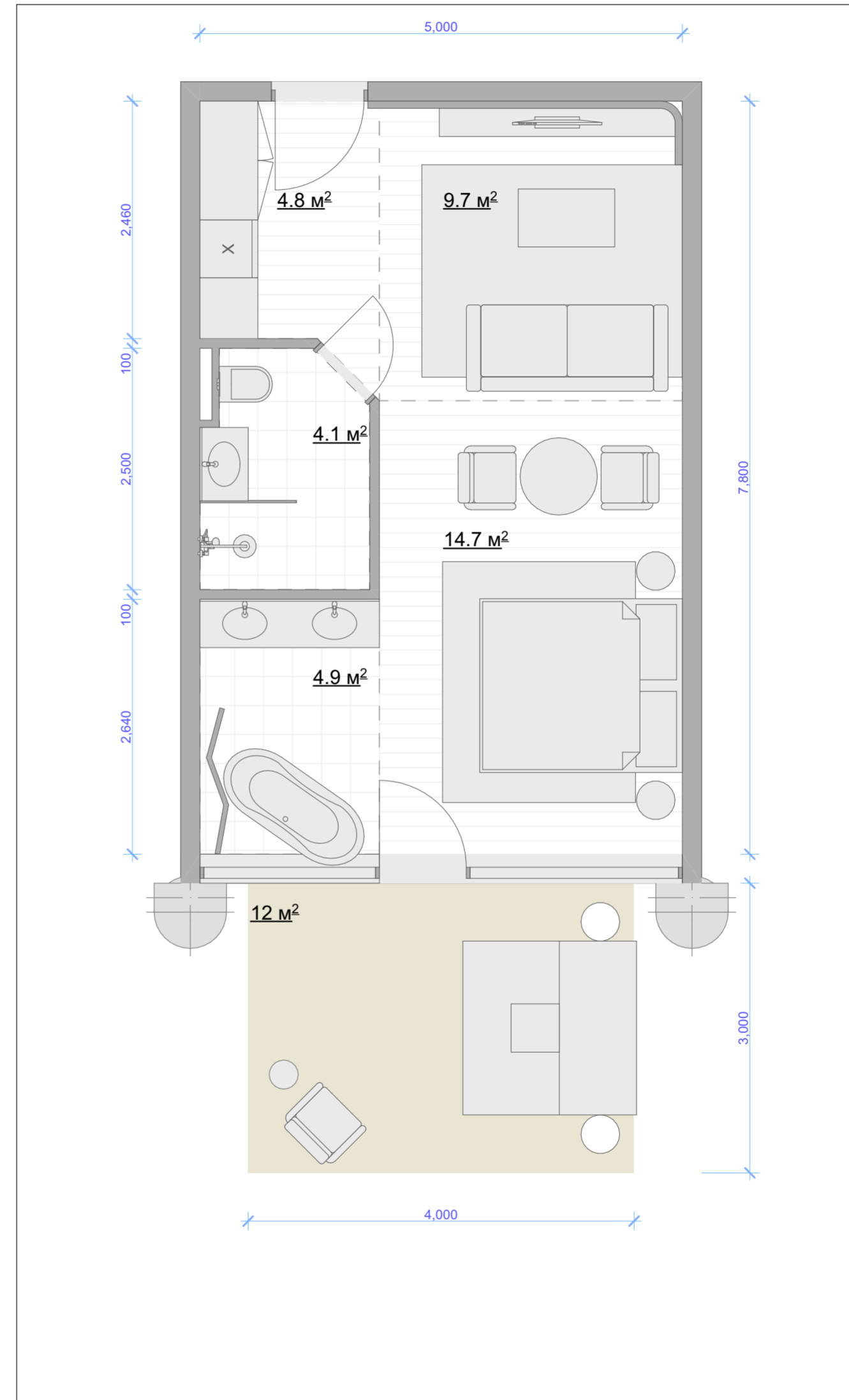
Deluxe room. Type 1 x2 38,2m 2 76,4m 2
