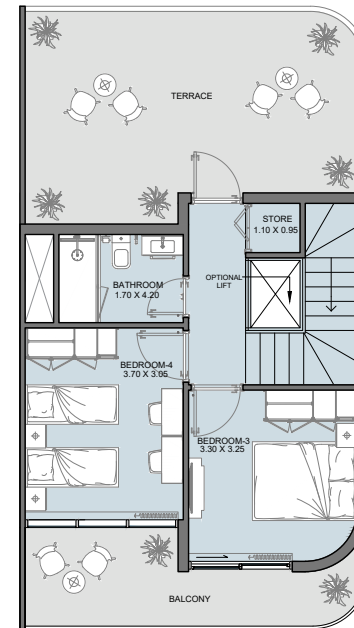
SECOND FLOOR Corner Unit
