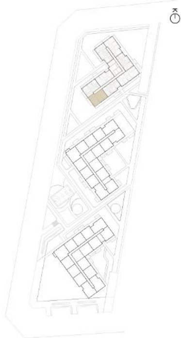
SITE PLAN
