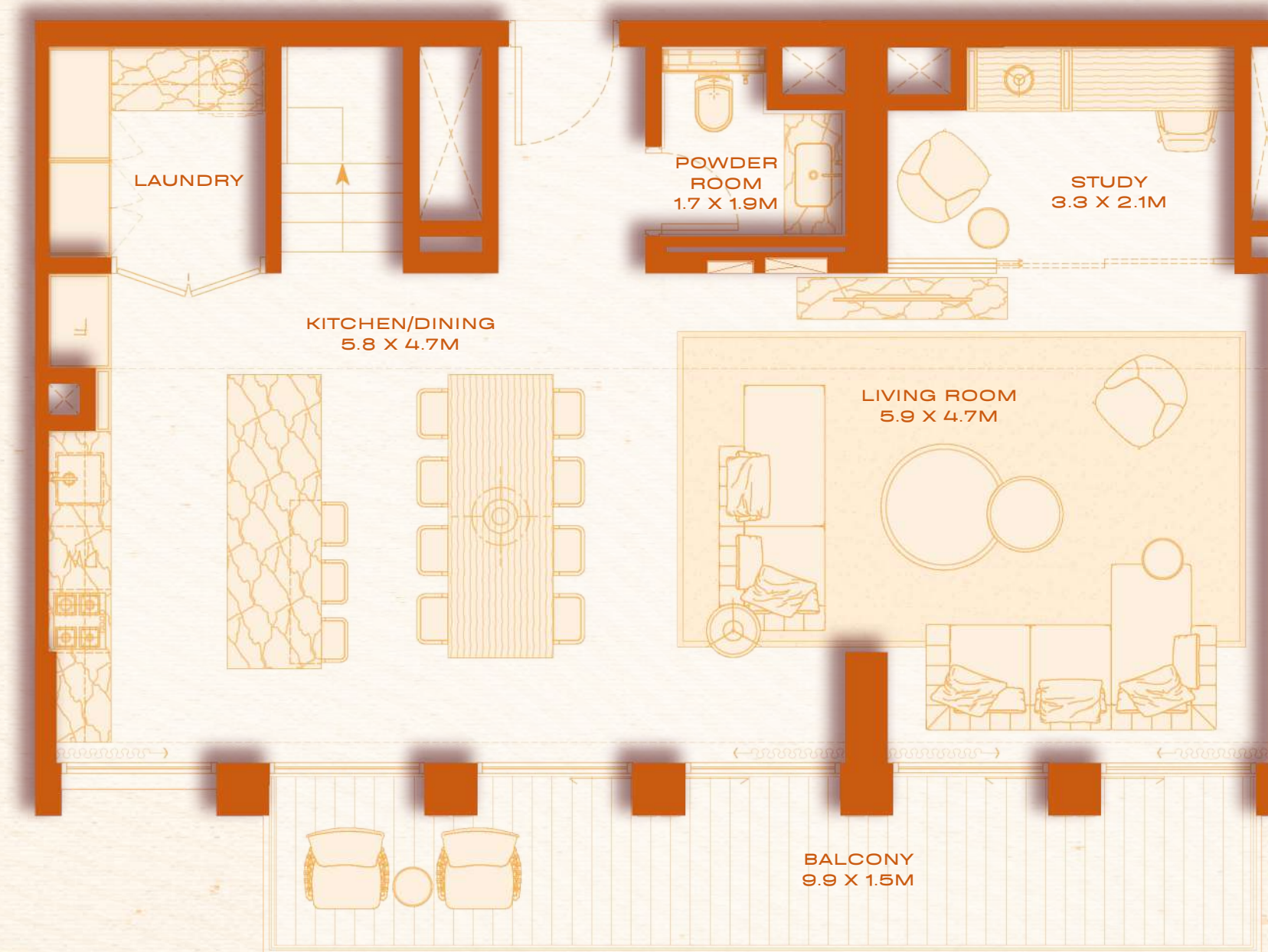
GROUND FLOOR
