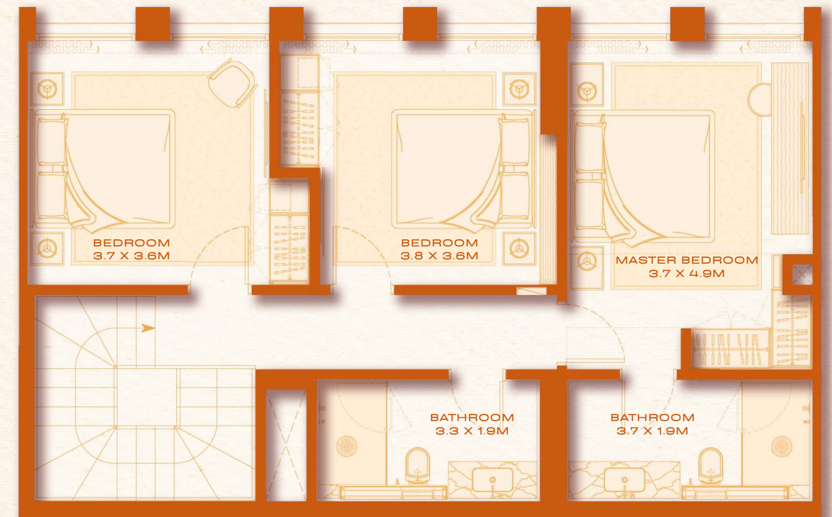
FIRST FLOOR
