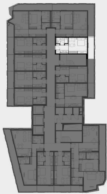
1-9 floor
