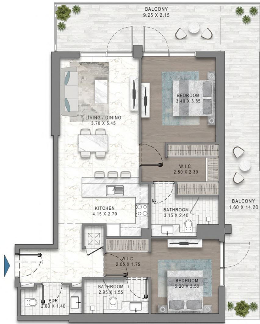
2BR - TYPE C1
