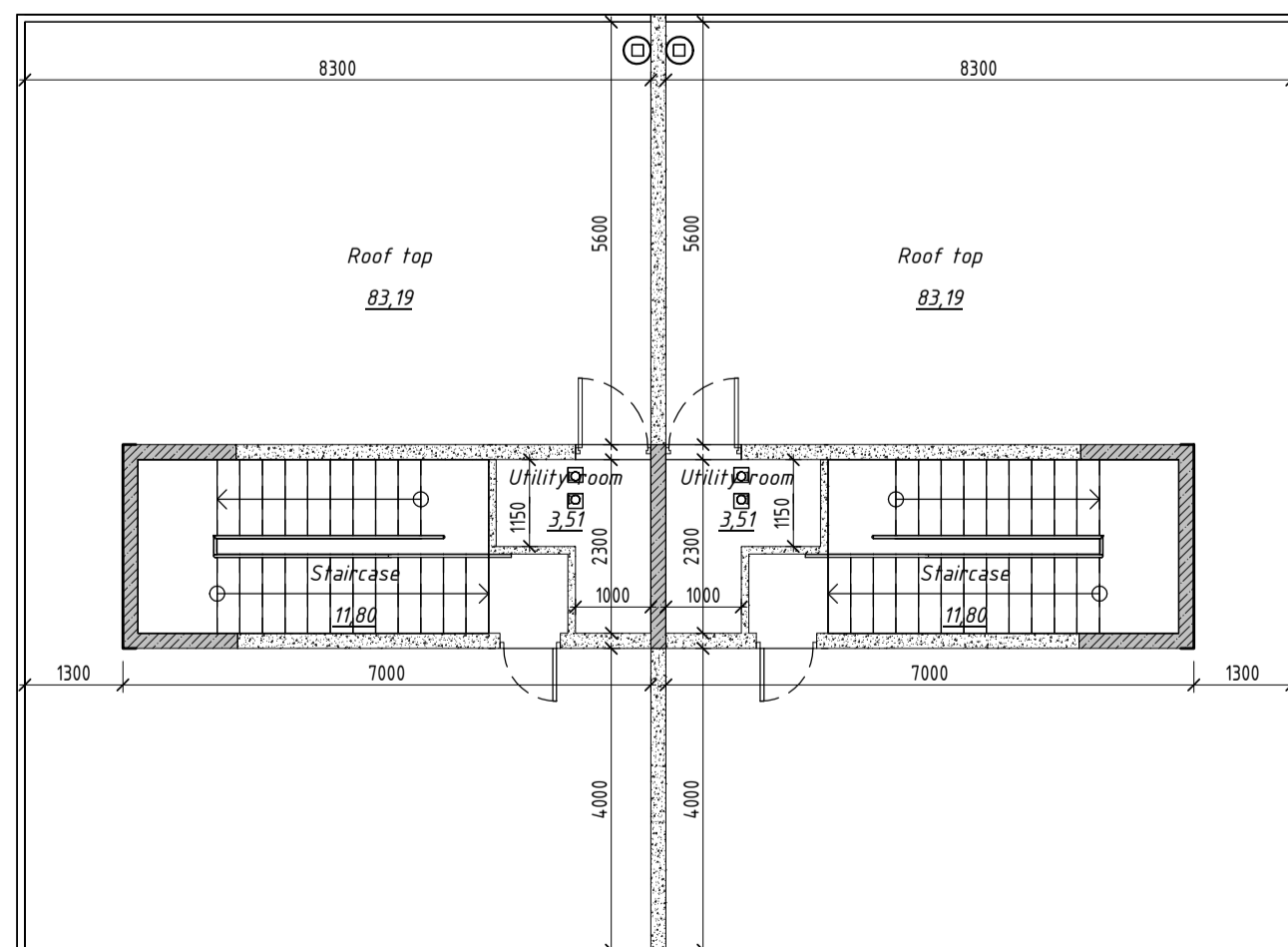
Roof Top
