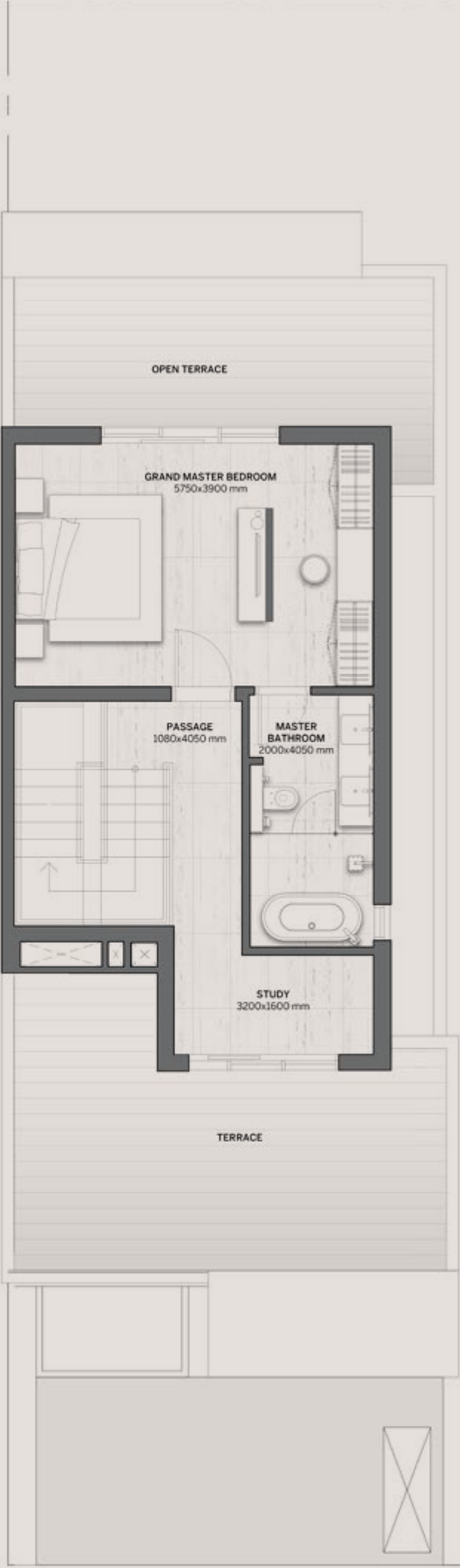
SECOND FLOOR
