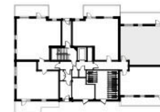
CRANEFORD HOUSE GROUND FLOOR – APARTMENT 2
