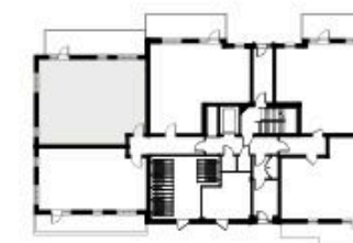
RIVIERA HOUSE GROUND FLOOR – APARTMENT 4
