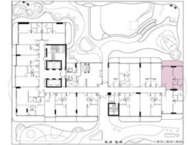
LEVEL 01 KEY PLAN
