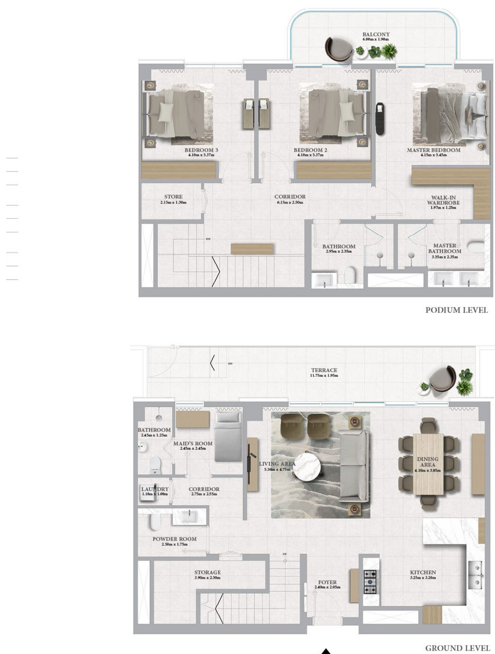
3-Bedroom Townhouse Layout
