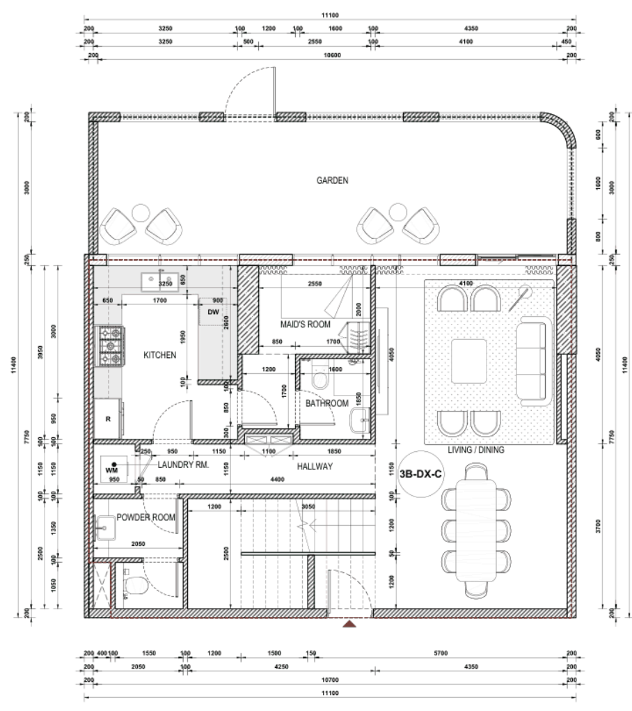
GROUND LEVEL
