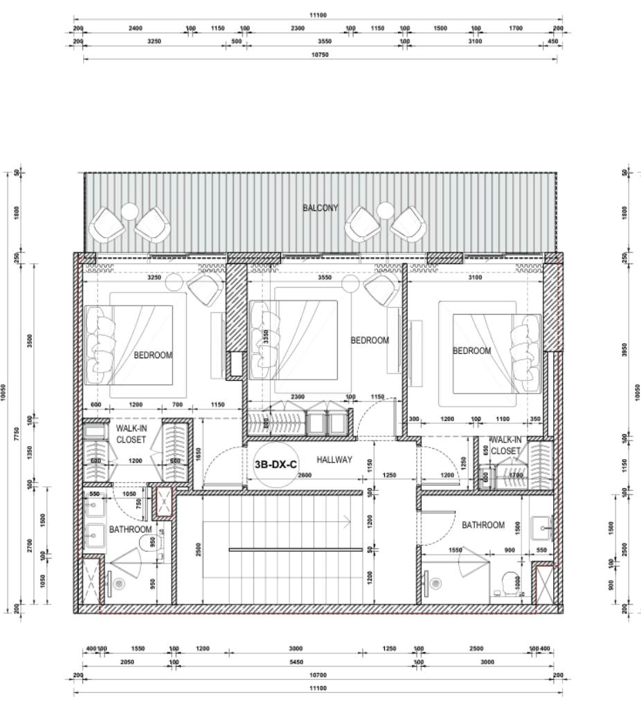
LEVEL 01
