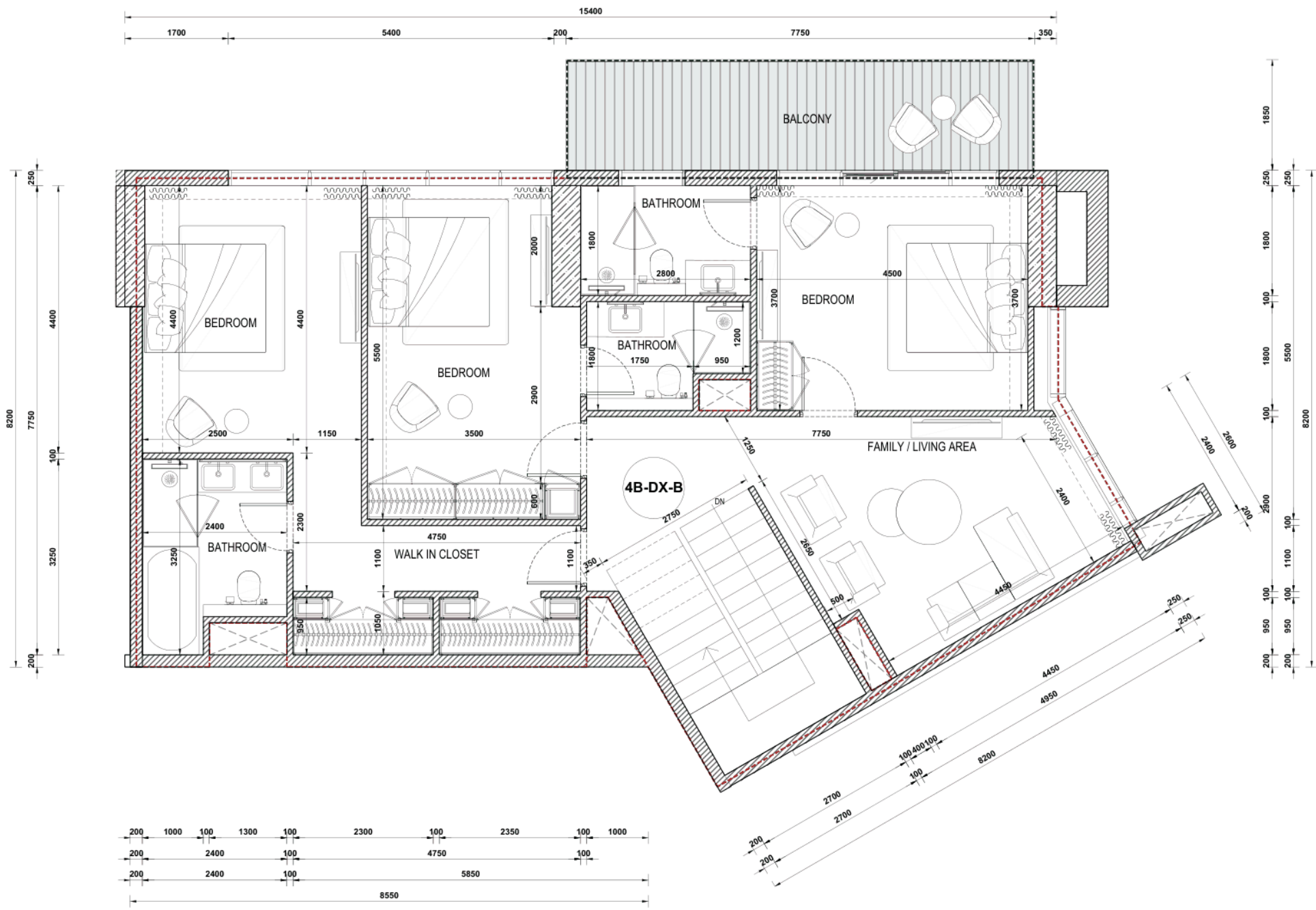
LEVEL 01
