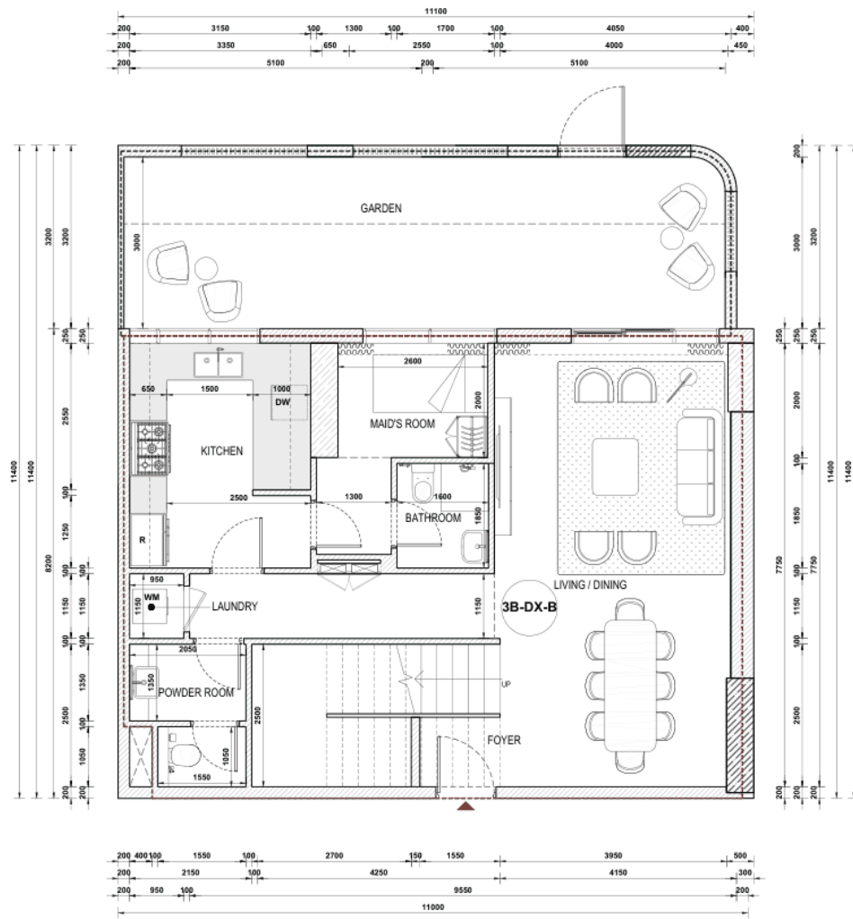
GROUND LEVEL
