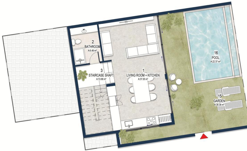
1 GF LEVEL GA PLAN 1 : 100
